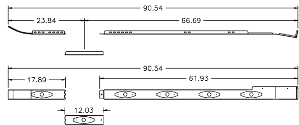
FUEL DOOR LOCATION - DRIVER
